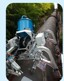
Automatic external UHP water jetting
